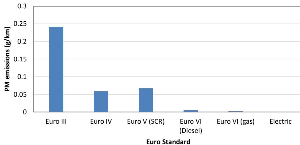
Figure 20 – PM emissions of buses by Euro Standard and fuel type (at 18km/hr)
